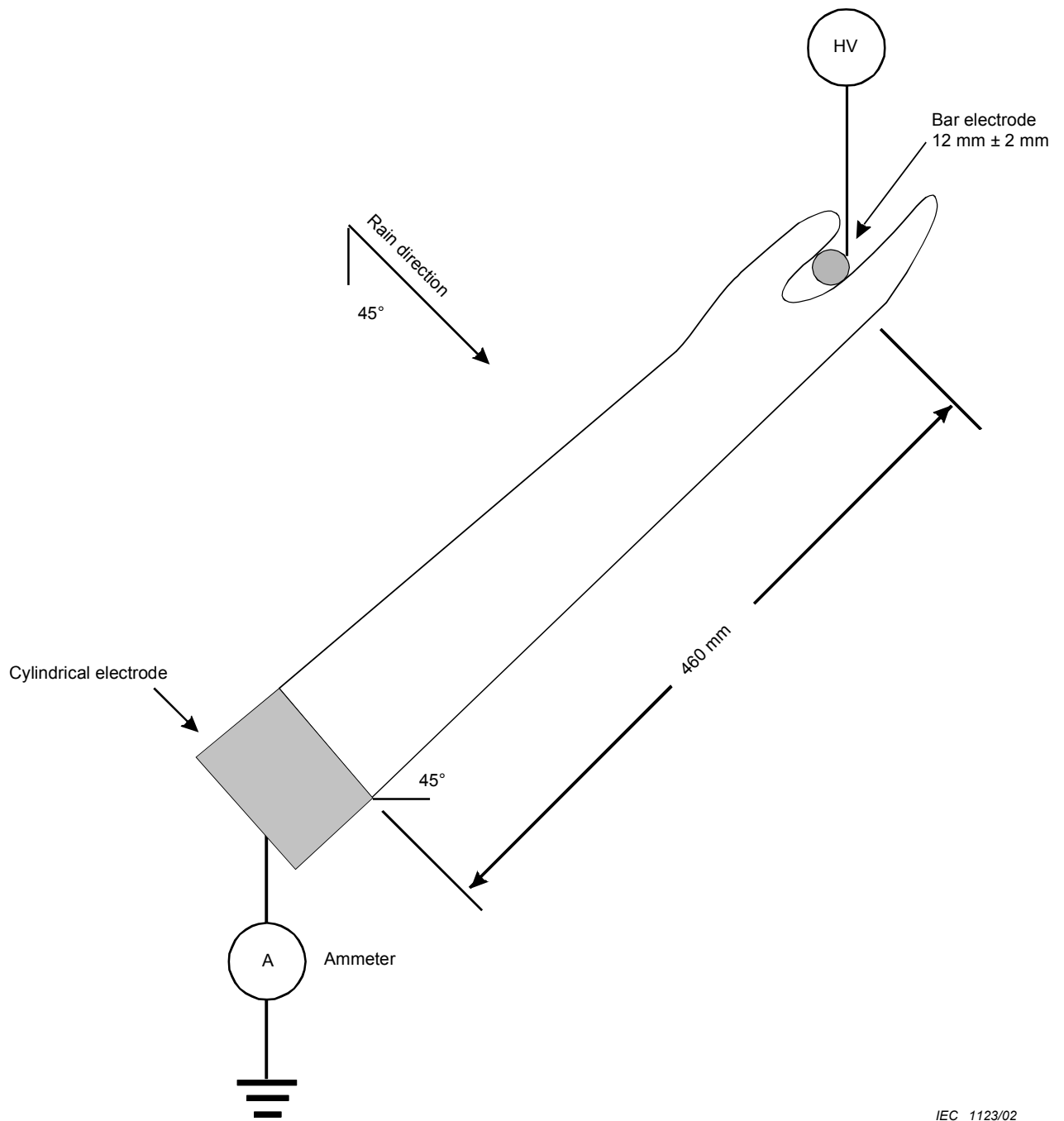
Figure 16 – Set-up for the leakage current test (see 10.2)
